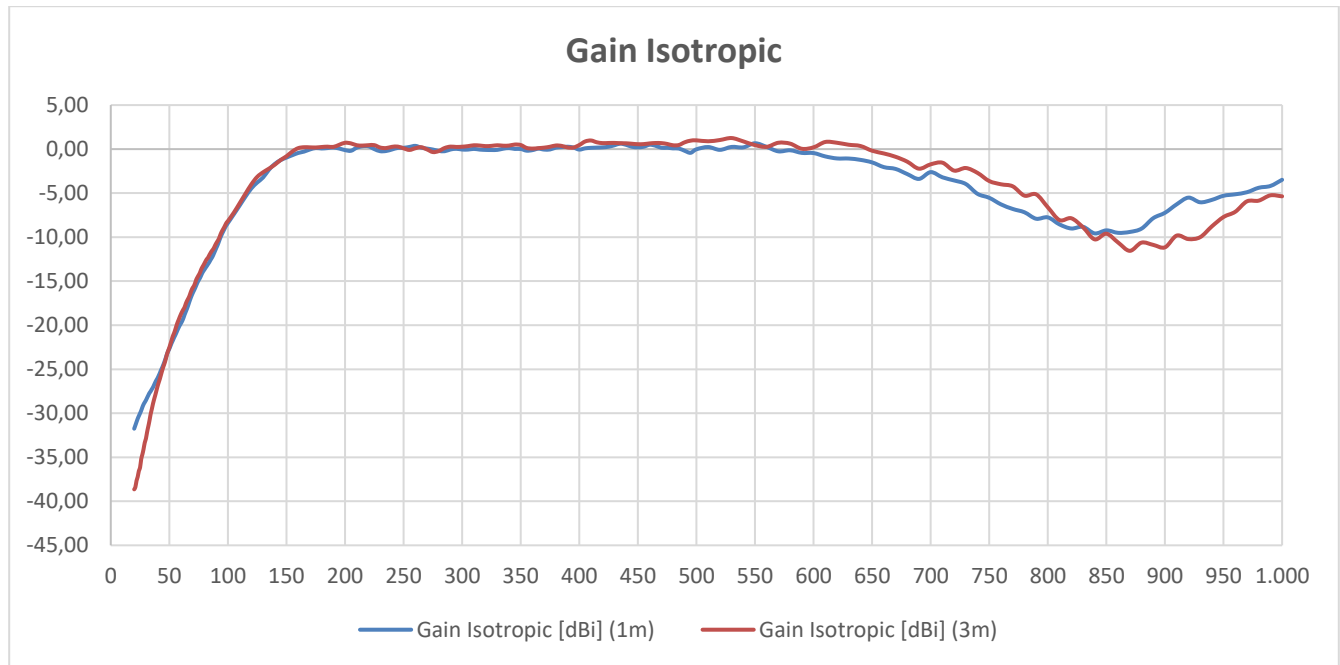
20 MHz ... 1000 MHz, Isotropic Gain of TBMA1C
