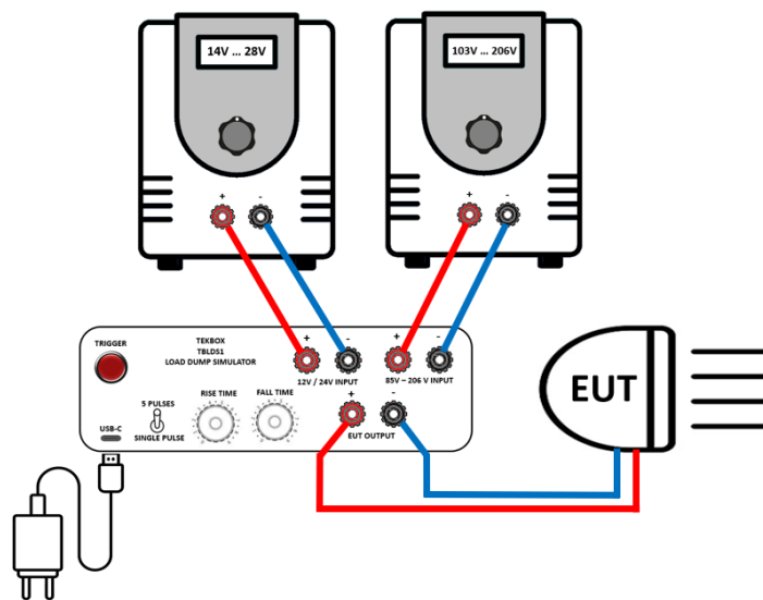
Test setup
