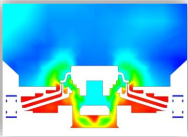
Without thermal refinement - Uneven heat distribution
