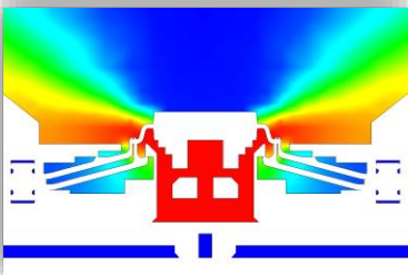
Precision thermal socket design - Consistent DUT temperature
